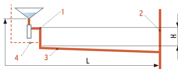
1 connection bend 2 downpipe 3 connection pipe 4 venting pipe
